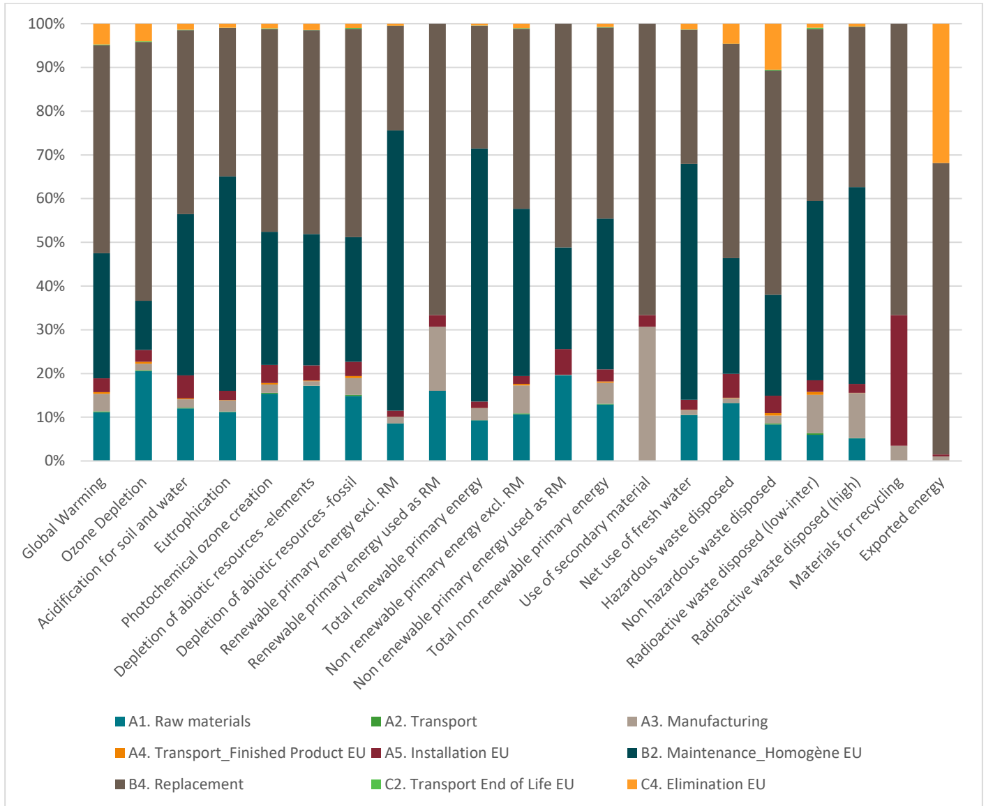
Figure 7: Graph depicting selection of impact indicator results calculated according to EN 15804 – Europe
